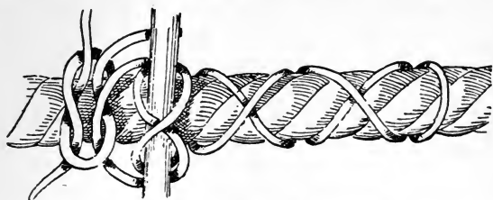
FIG. 47.—Chain hitch with bar.
